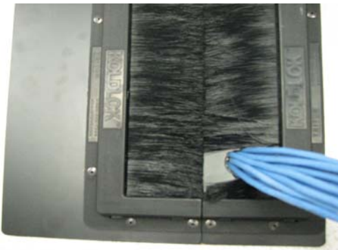
Figure 4. The position of cable bundles in brush-style grommets can move bristles out of position to reduce sealing effectiveness. In addition, bristles can sag, degrade, or break off over time.
