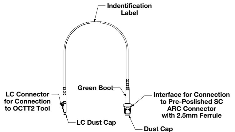
2.5mm SM APC Fiber Optic Launch Cord
