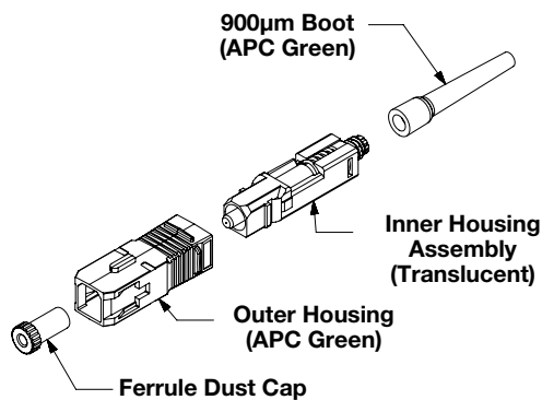
OptiCam SC APC Connector
