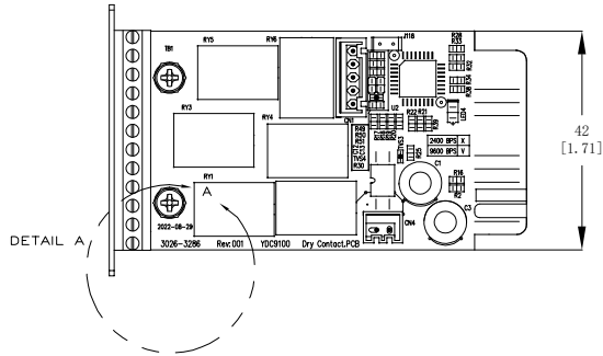
DETAIL A: 3026-3286 Rev:001 YDC9100 DRY CONTACT PCB
