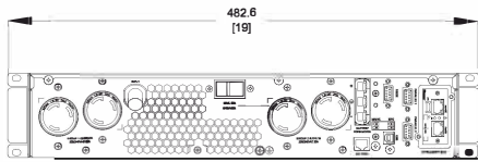
VIEW ROTATED 180°
