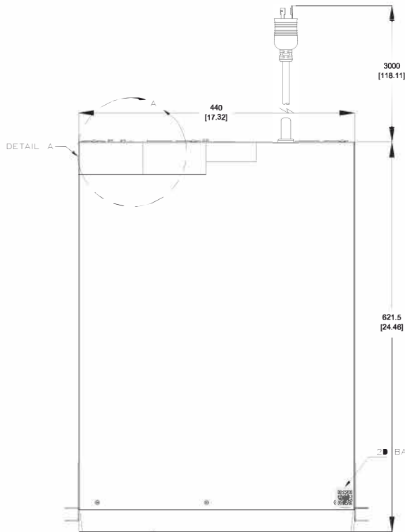
VIEW ROTATED 180°
