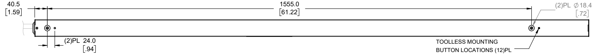
REAR VIEW
