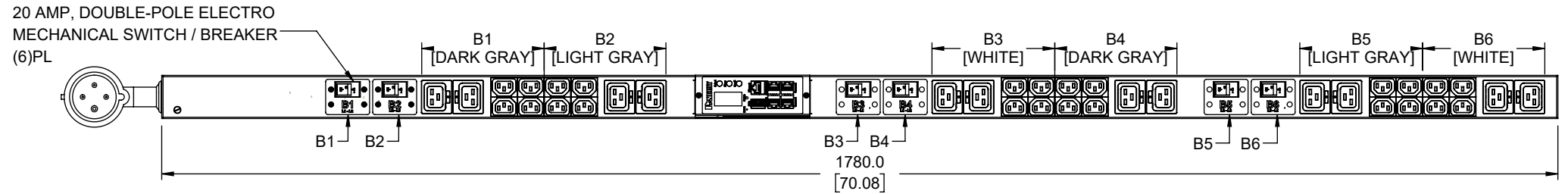
FRONT VIEW
